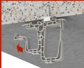
Simply click the cable clamp on to the satellite, either on the wall or ceiling.
